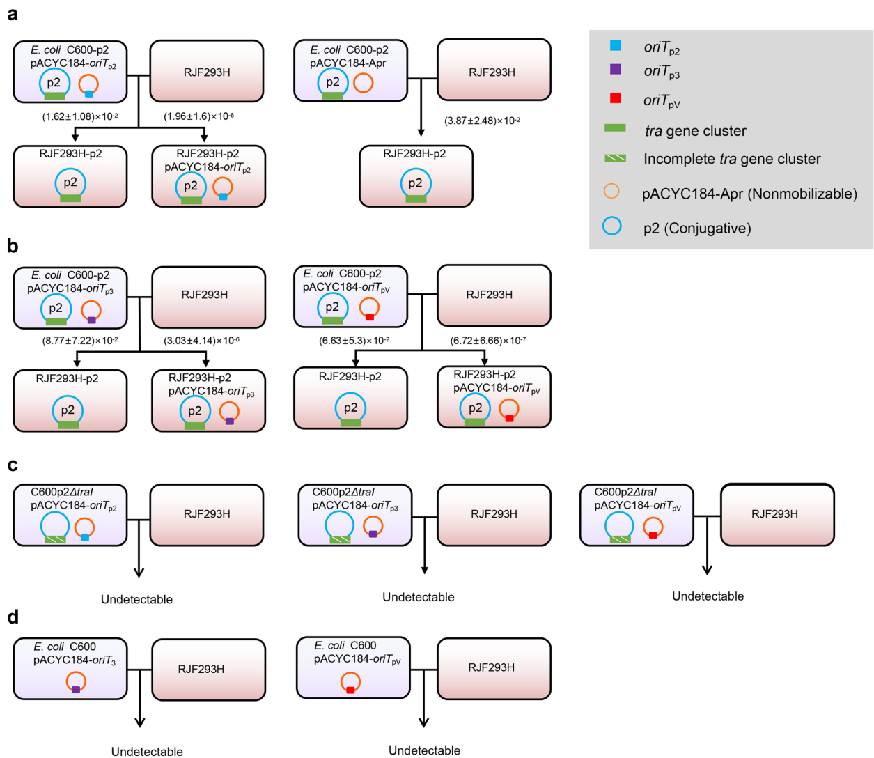
Fig. 3 Schematic diagram of the simulation of mobilization of the virulence plasmid pRJF293 (pV) and the MDR plasmid pKPHS3 (p3) with their oriTs and the help of the CR plasmid pKPHS2 (p2). a When accompanied by pKPHS2, pACYC184- oriT p2 can be transferred while the empty vector pACYC184 cannot. b When accompanied by plasmid pKPHS2, pACYC184- oriT p3 and pACYC184- oriT pV can be transferred. c pACYC184- oriT p2 , pACYC184- oriT p3 , and pACYC184- oriT pV cannot be transferred when accompanied by plasmid pKPHS2Δ tral . d pACYC184- oriT p3 and pACYC184- oriT pV cannot be transferred alone. The orange circle denotes the backbone of plasmid pACYC184- Apr , and the blue circle denotes the conjugative plasmid pKPHS2. The green square denotes the tra gene cluster. The blue square denotes the oriT derived from plasmid pKPHS2. The purple square denotes the oriT derived from pKPHS3. The red square denotes the oriT derived from pRJF293. The conjugative frequencies of detected transconjugants that acquired either pKPHS2 (p2) or both pKPHS2 (p2) and pACYC184 derivatives are listed. Detailed data are available in Additional file 6: Table S5
